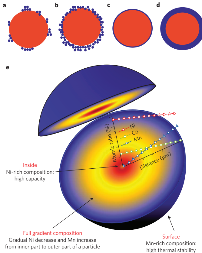
Figure 3 | Schematics of strategies to protect cathodes from reacting with non-aqueous electrolytes. a–e. Rough particulate coating (a), thin homogeneous coating (b), ultra-thin surface coating by atomic layer deposition (c), core-shell structure using manganese-rich shell to protect the nickel-rich core (d) and full concentration gradient cathodes with the concentration of nickel continuously decreasing from the centre to the surface (e). Panel e reproduced from ref. 35, NPG.
